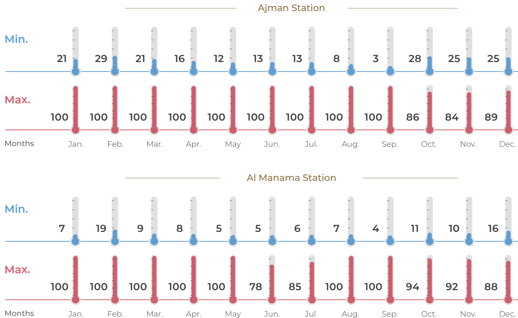
Figure (17-4): Maximum and Minimum of Relative Humidity by month and station in the Emirate of Ajman during the year 2024
