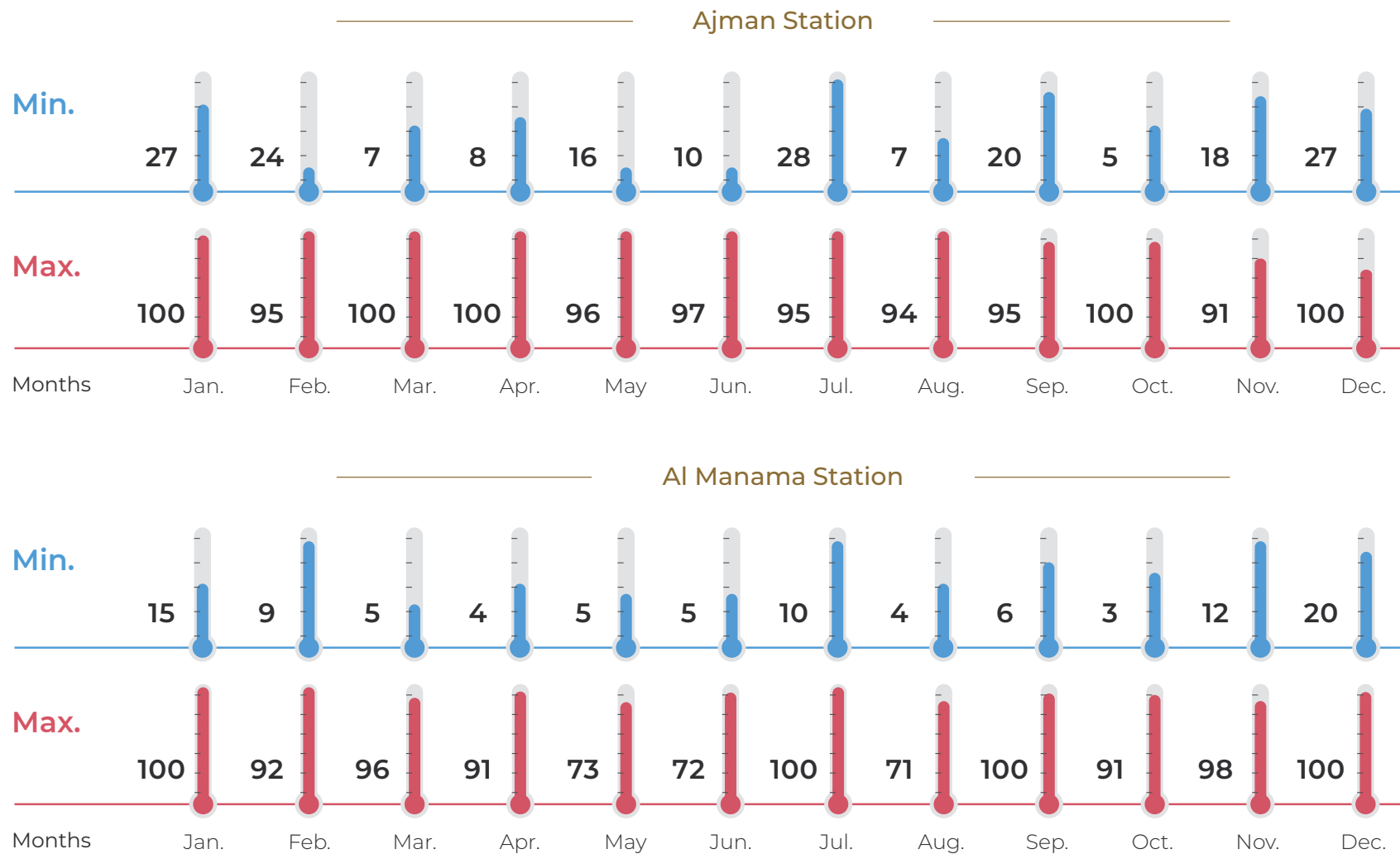
Figure (18-4): Maximum and Minimum of Relative Humidity by Month and Station in the Emirate of Ajman during the Year 2022
