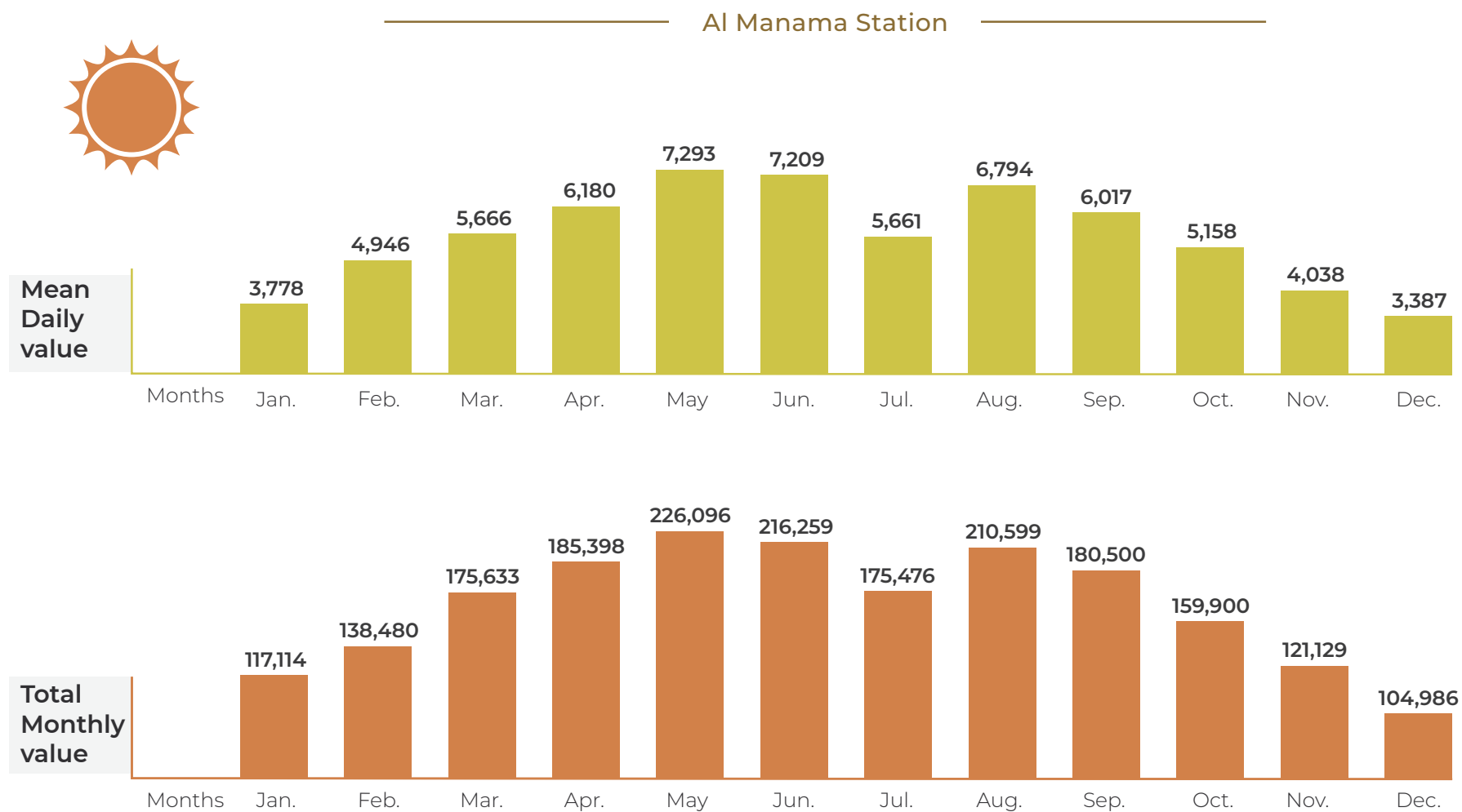
Figure (18-8): Daily Mean and Total Monthly of Solar Radiation by Month & Station in the Emirate of Ajman during the year 2022
