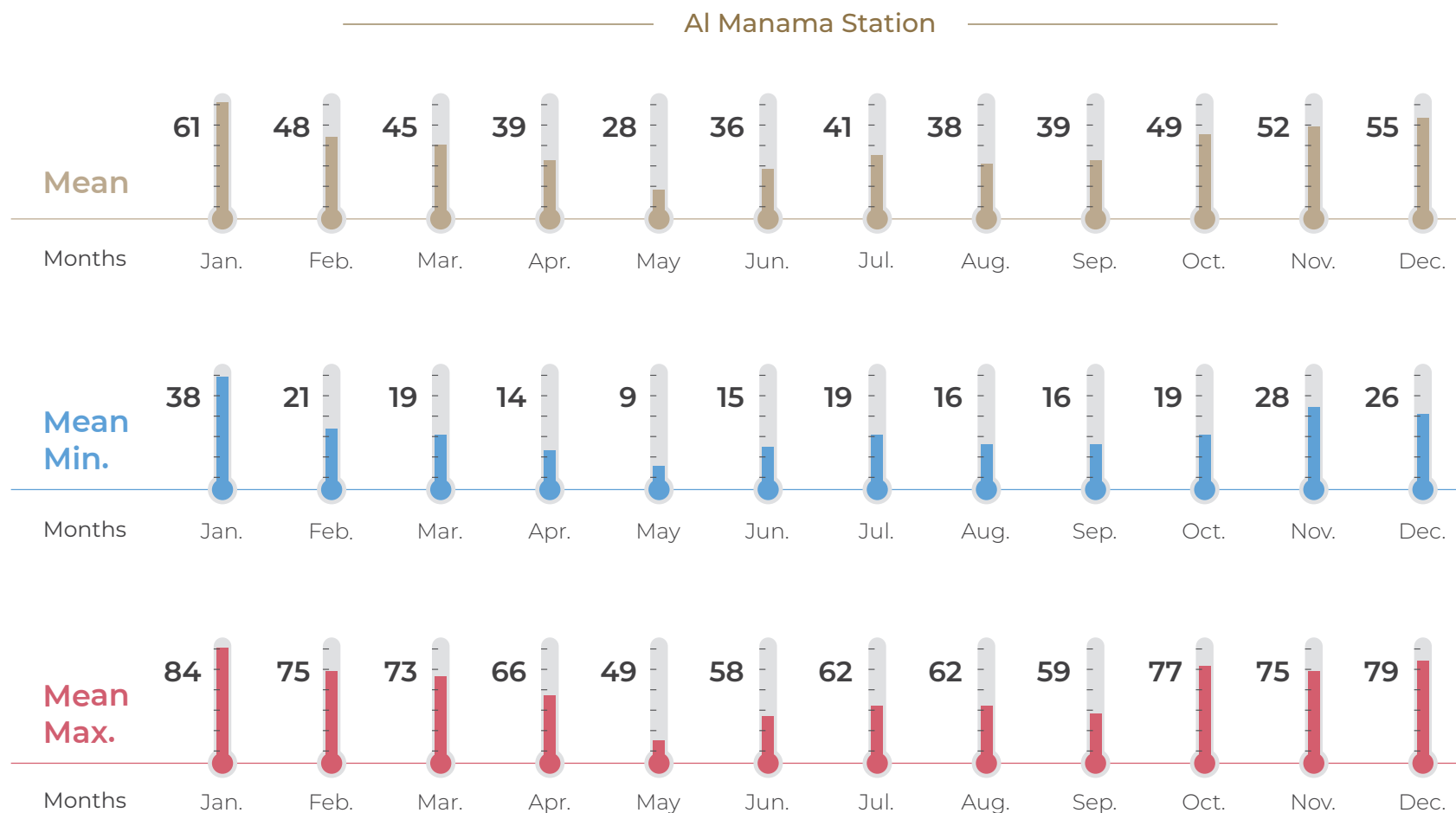
Continued... Figure (17-5): Mean Minimum and Maximum Average of Relative Humidity by Month & Station in the Emirate of Ajman during the Year 2023
