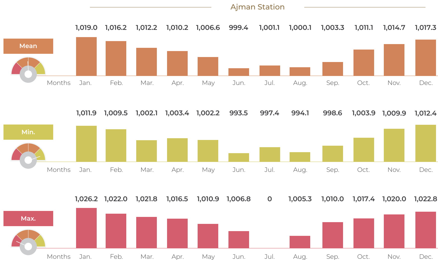
Figure (17-6): Measurements of Atmospheric Pressure at Sea Level by Month and Station in the Emirate of Ajman during the Year 2023
